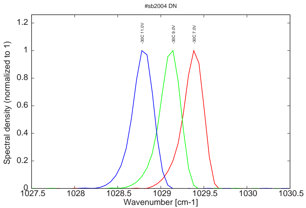
Figure 9: spectra at -30C for various LDD voltages at 2% duty-cycle (monomode range)
