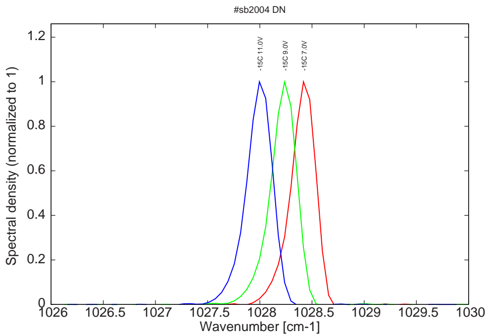
Figure 11: spectra at -15C for various LDD voltages at 2% duty-cycle (monomode range)
