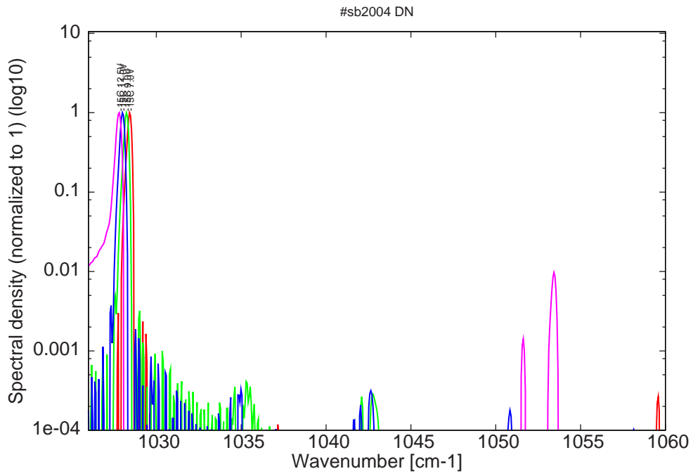
Figure 10: spectra at -15C for various LDD voltages at 2% duty-cycle
