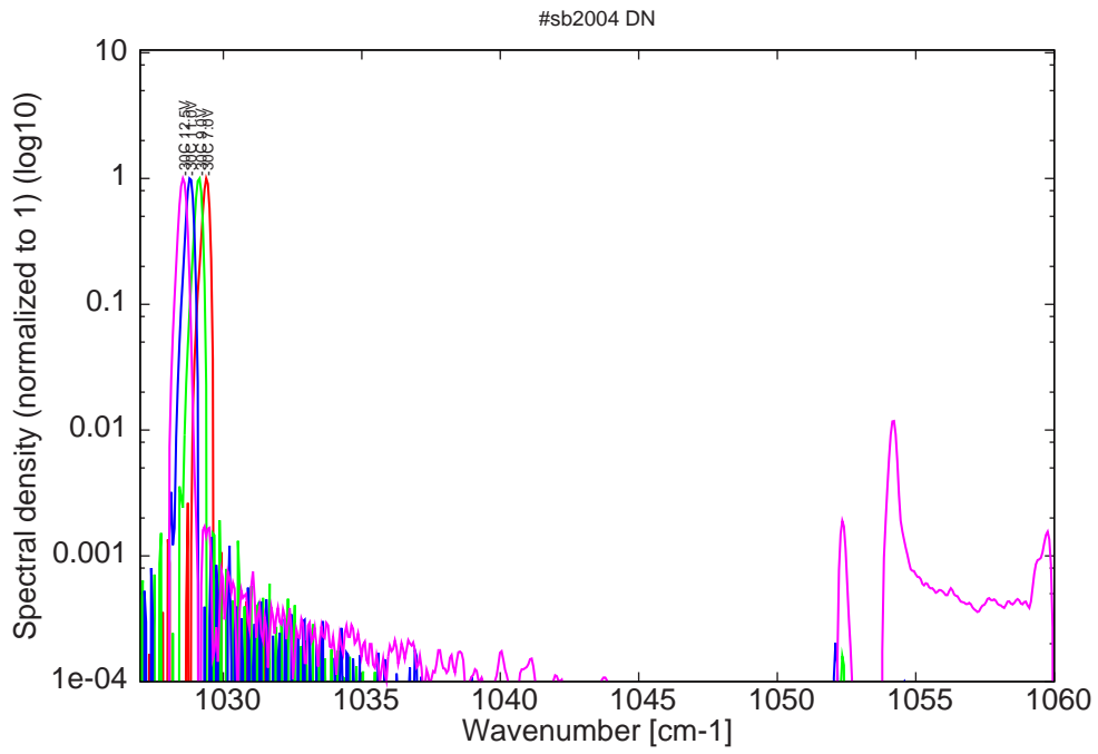
Figure 8: spectra at -30C for various LDD voltages at 2% duty-cycle
