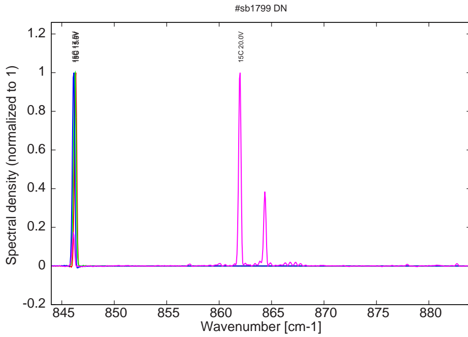
Figure 14: spectra at 15C for various LDD voltages
