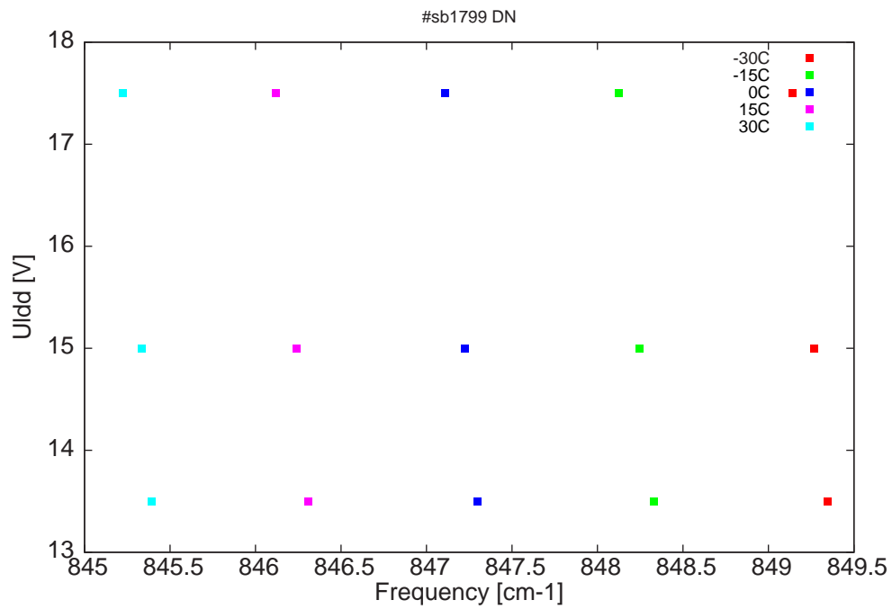
Figure 3: DC voltage fed to LDD ( U_{idd} ) as a function of the singlemode emission frequencies and temperatures
