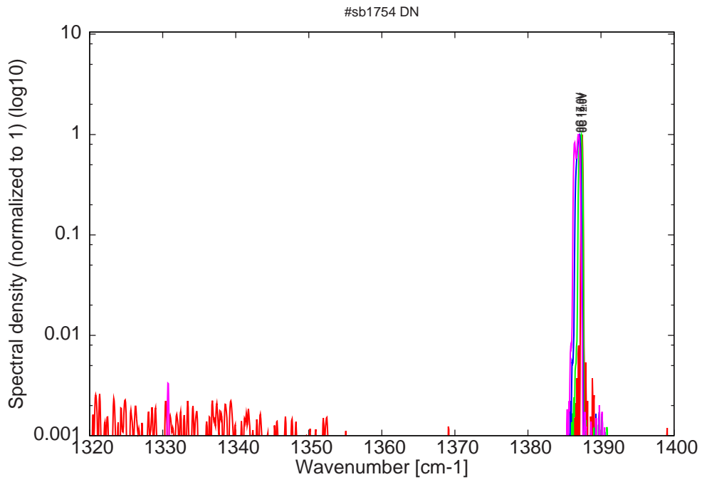
Figure 12: spectra at 0C for various LDD voltages; monomode up to 16V
