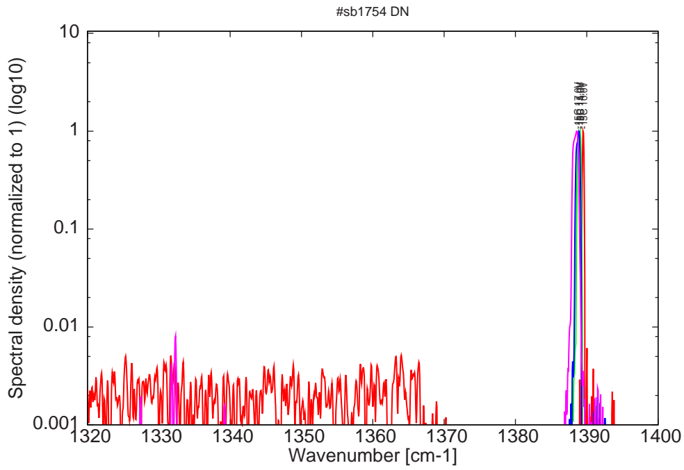
Figure 10: spectra at -15C for various LDD voltages; monomode up to 15V
