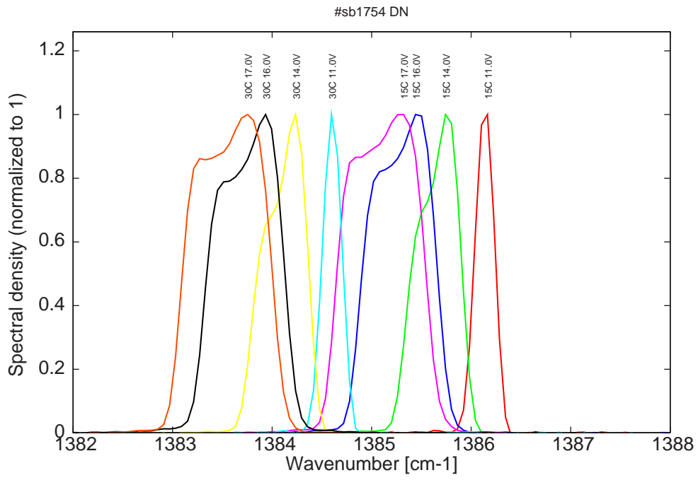
Figure 14: spectra at 15C and 30C for various LDD voltages; all monomode
