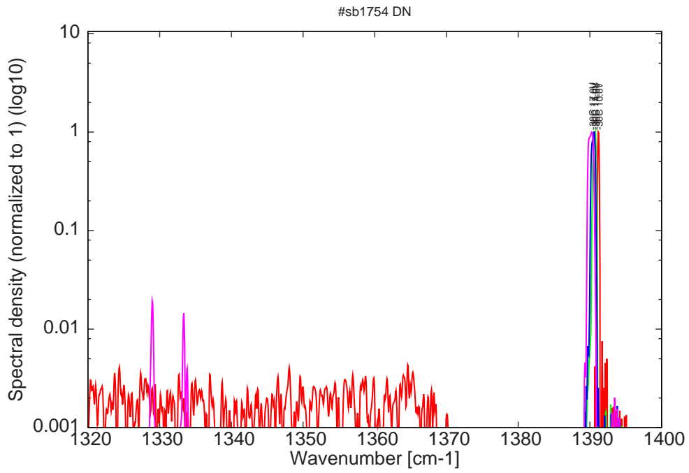
Figure 8: spectra at -30C for various LDD voltages; monomode up to 15V
