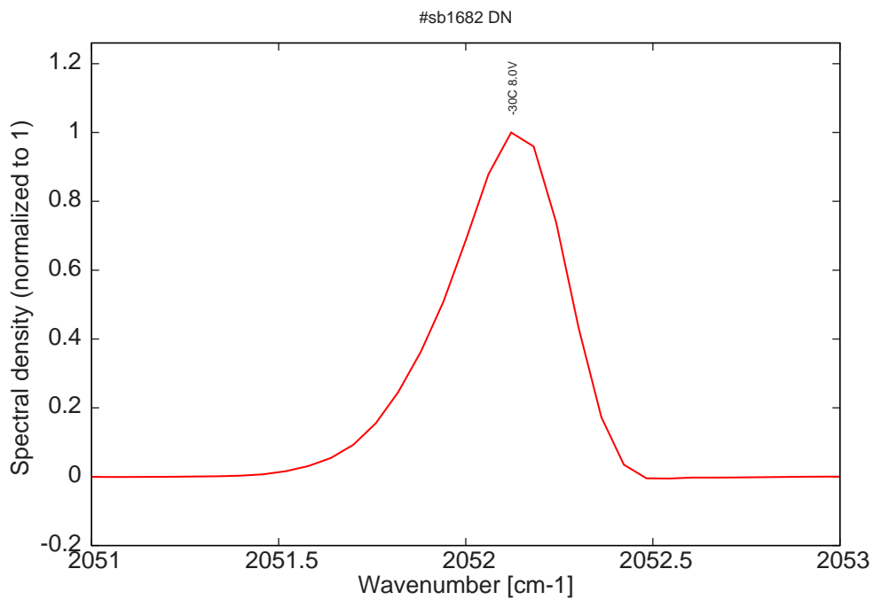
Figure 9: monomode spectrum at -30C and 8.0V on LDD
