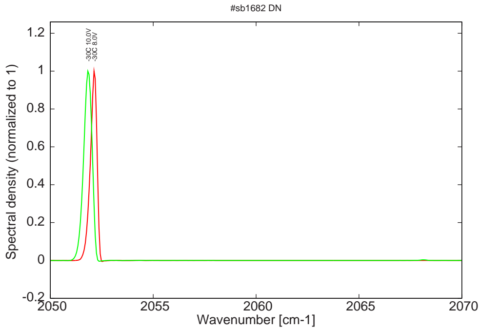
Figure 8: spectra at -30C for various LDD voltages (small mode around 2069.5 cm-1 for more than 10.0V on LDD)
