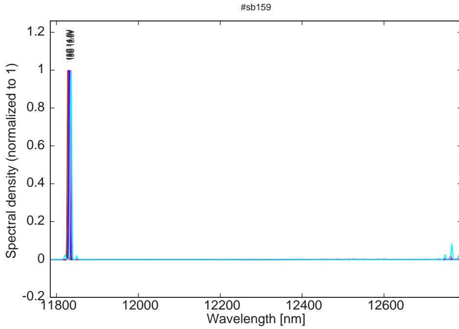
Figure 15: spectra at 15C for various LDD voltage
