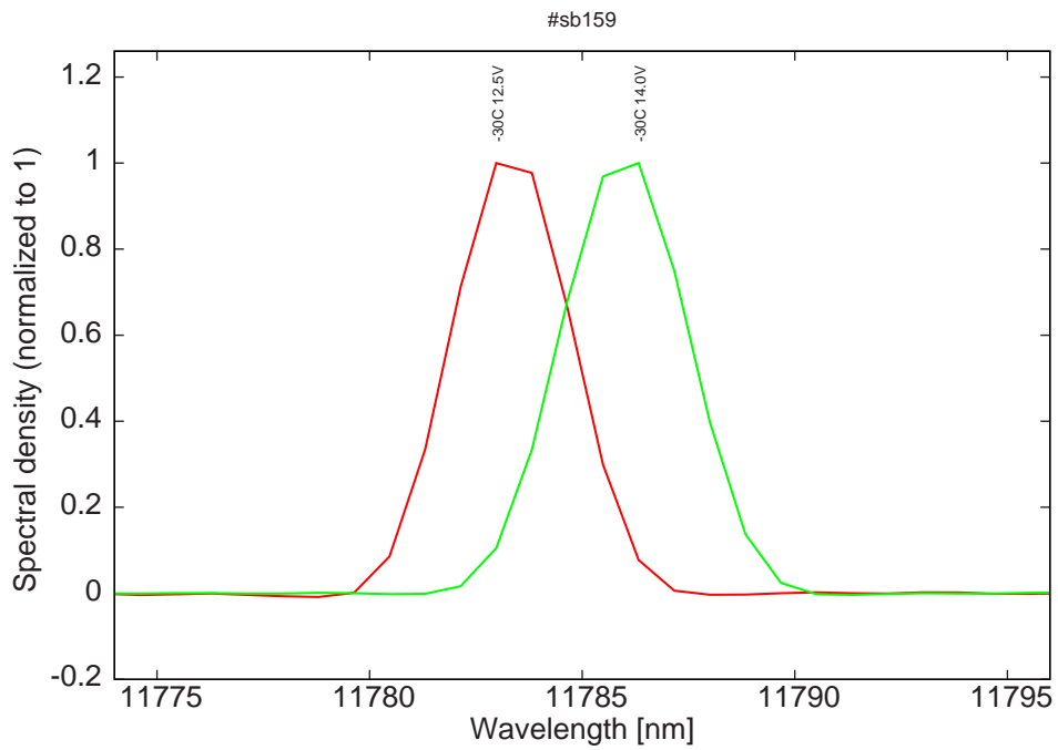
Figure 10: spectra at -30C for various LDD voltage (monomode range)
