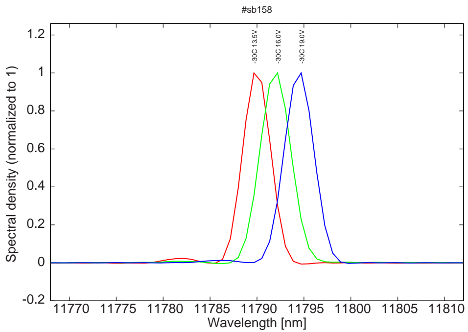
Figure 10: spectra at -30C for various LDD voltage (bimode range)
