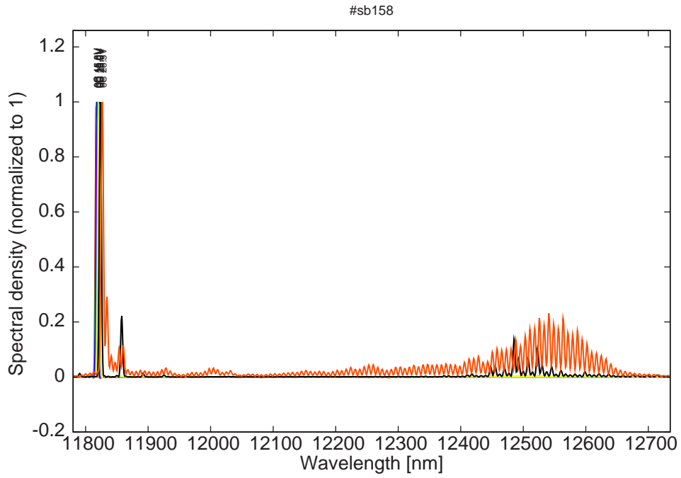
Figure 13: spectra at 0C for various LDD voltage
