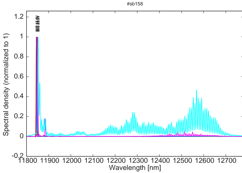
Figure 17: spectra at 30C for various LDD voltage
