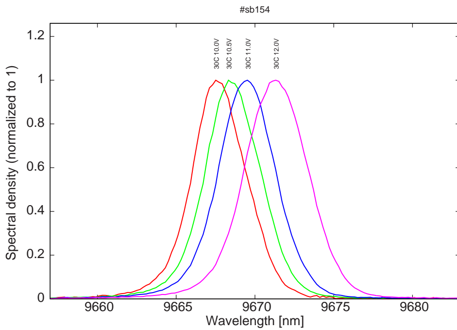
Figure 16: spectra at 30C for various LDD voltage (monomode)
