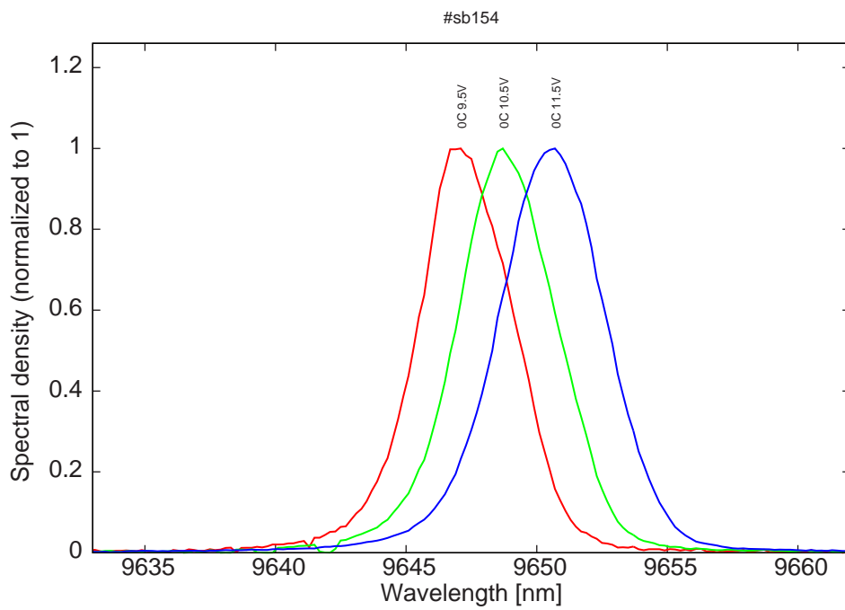
Figure 14: spectra monomodes at 0C for various LDD voltage (monomode range)
