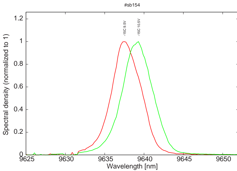
Figure 12: spectra monomodes at -15C for various LDD voltage (monomode range)
