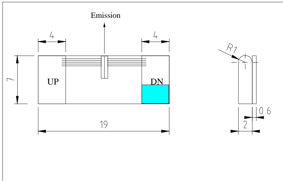
Figure 1: Mechanical and electrical interface for #sb154 DN (please note that the laser is connected to the DN pad drawn in blue)
