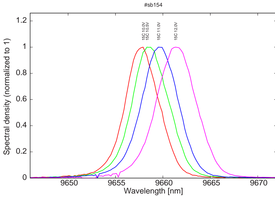
Figure 15: spectra at 15C for various LDD voltage (monomode)
