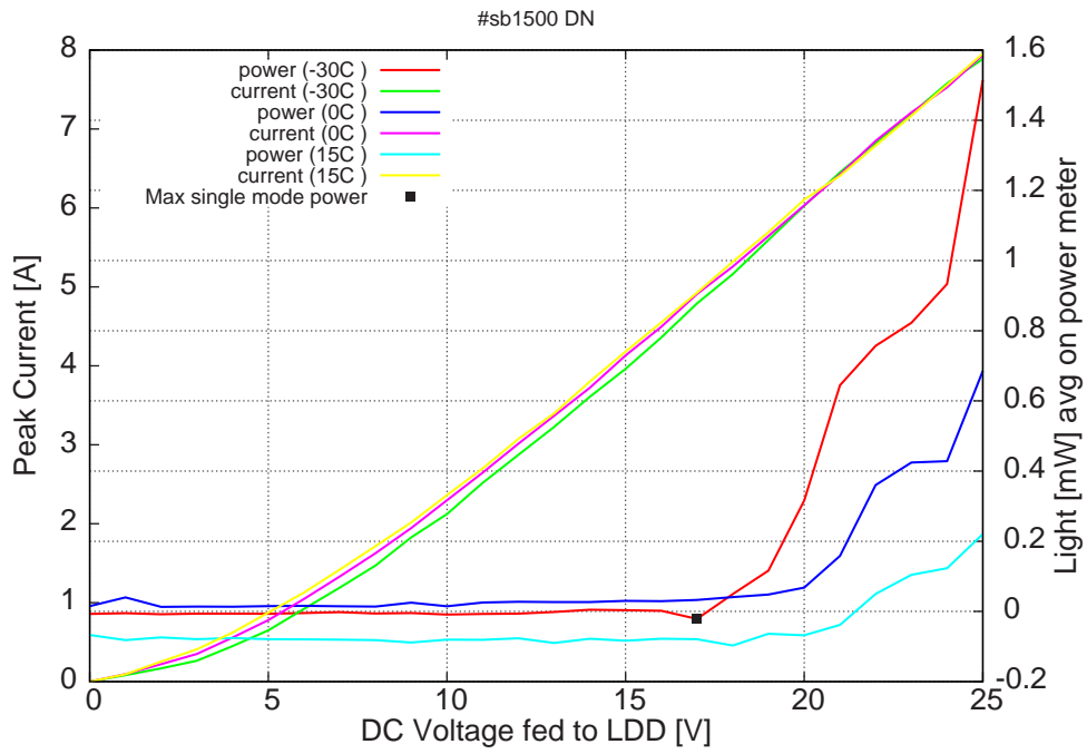
Figure 7: peak current and average power vs LDD voltage at 2% duty-cycle (50ns pulses, 2.5\mu\text{s} period) (including the multimode region)
