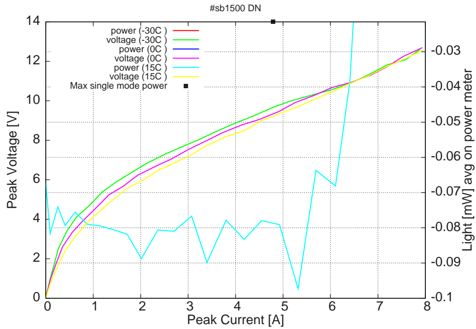
Figure 4: peak voltage and average power vs peak current at 2% duty-cycle (50ns pulses, 2.5\mu\text{s} period) (the solid squares indicate the maximum singlemode emitted power)
