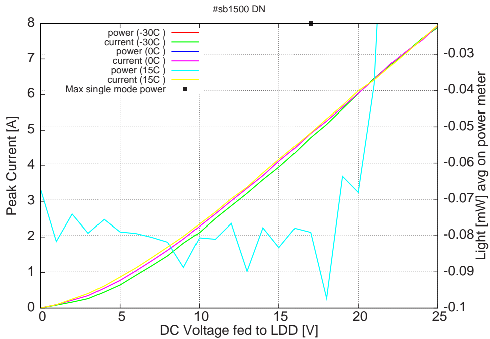
Figure 6: peak current and average power vs LDD voltage at 2% duty-cycle (50ns pulses, 2.5\mu\text{s} period) (the solid squares indicate the maximum singlemode emitted power)
