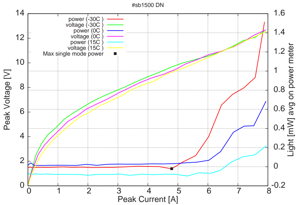
Figure 5: peak voltage and average power vs peak current at 2% duty-cycle (50ns pulses, 2.5\mu\text{s} period) (including the multimode region)
