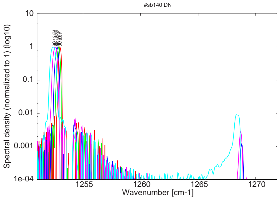
Figure 12: spectra at 0C for various LDD voltages (monomode up to 9V on LDD)
