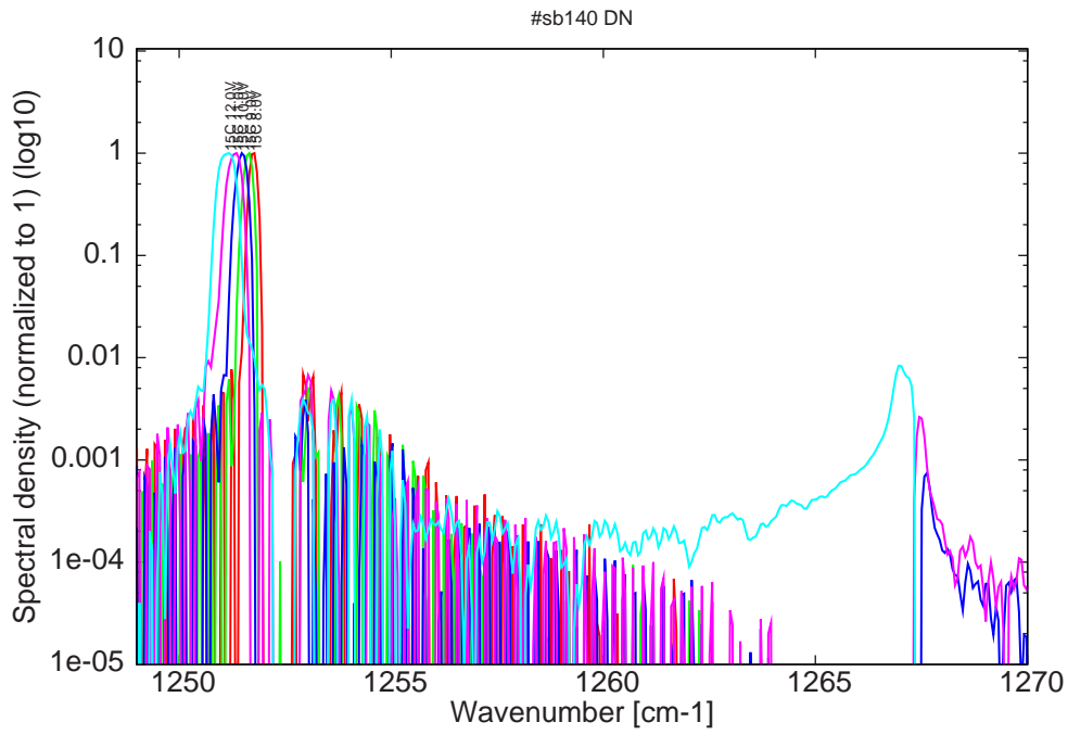
Figure 14: spectra at 15C for various LDD voltages (monomode up to 9V on LDD)
