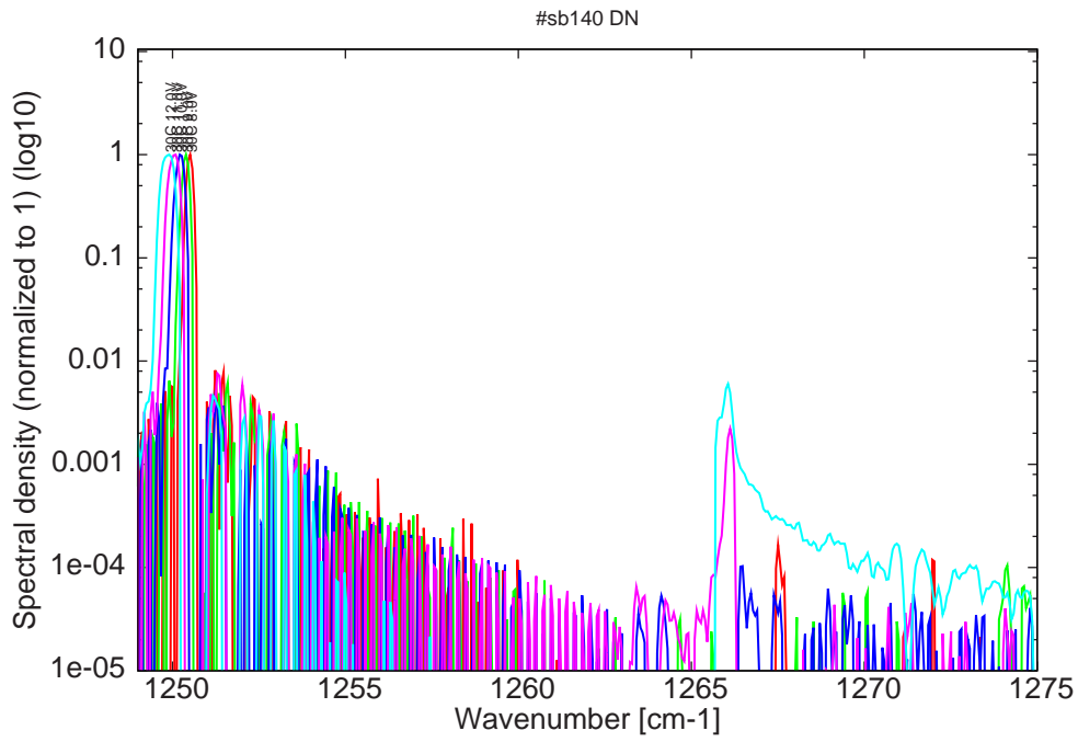
Figure 16: spectra at 30C for various LDD voltages (monomode up to 9V on LDD)
