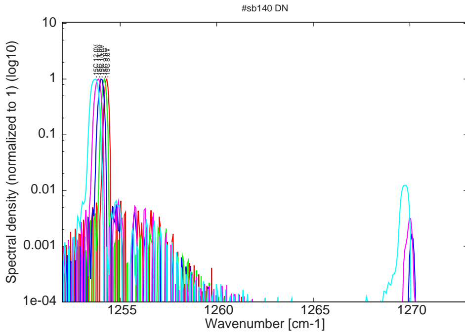
Figure 10: spectra at -15C for various LDD voltages (monomode up to 9V on LDD)
