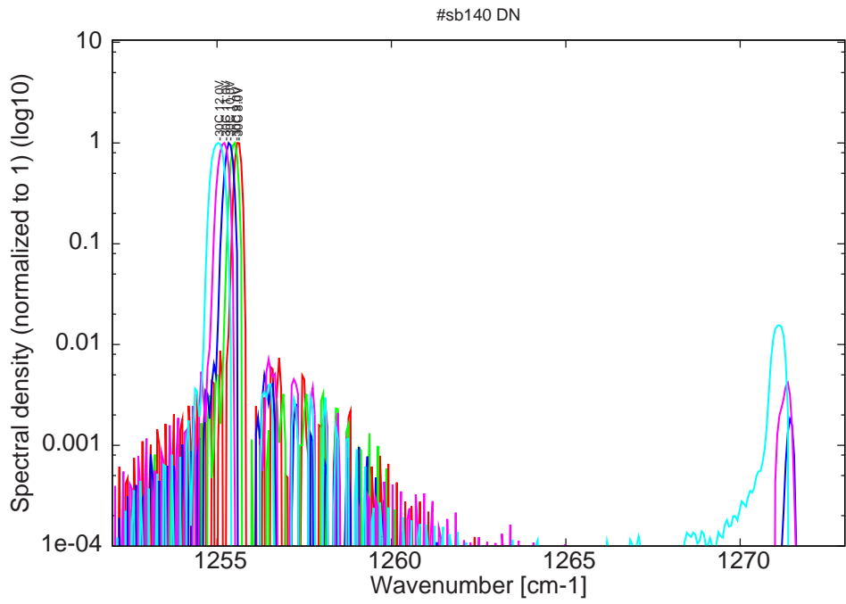
Figure 8: spectra at -30C for various LDD voltages (monomode up to 9V on LDD)
