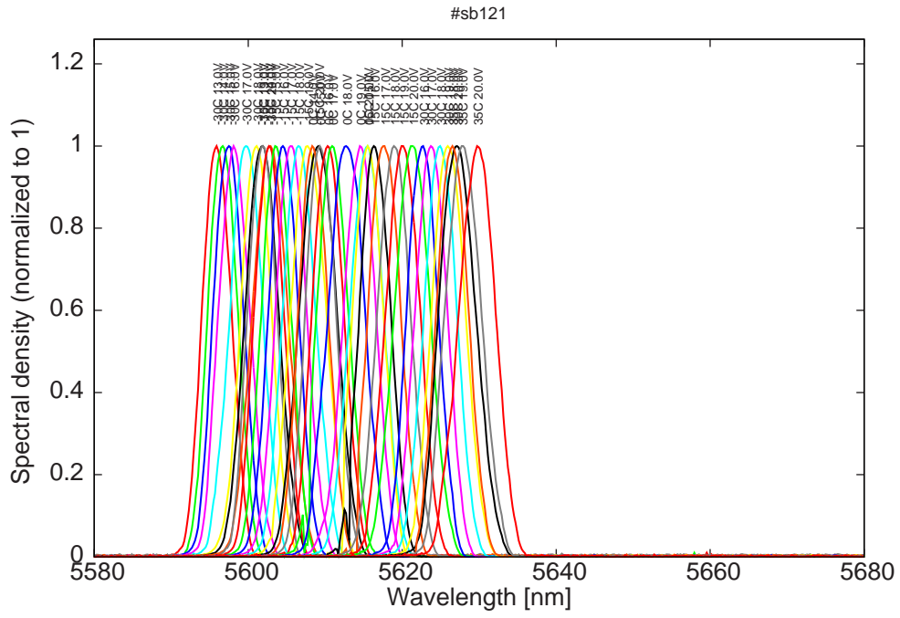
Figure 6: spectra at -30C, -15C, 0C, 15C, 30C and 35C for various LDD voltages
