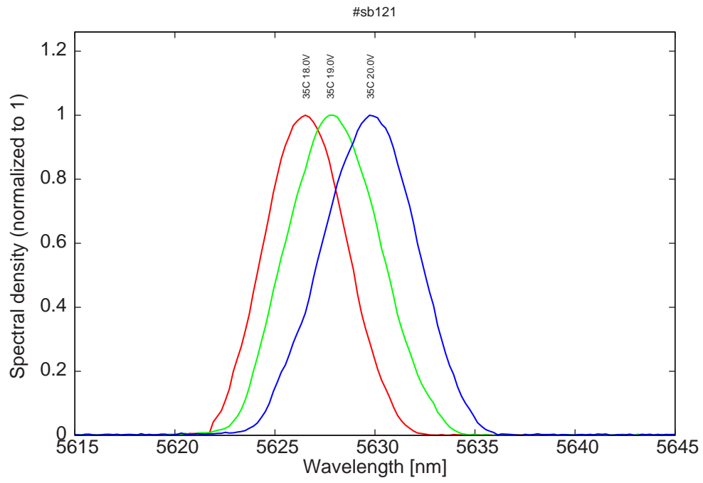
Figure 12: spectra at 35C for various LDD voltages
