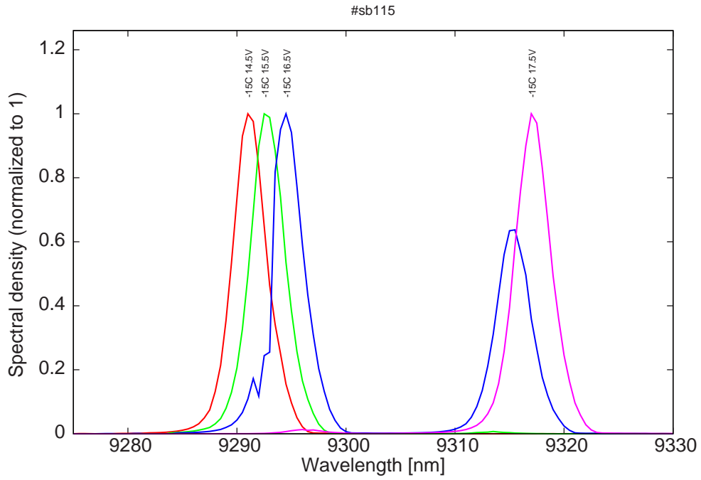
Figure 11: spectra at -15C for various LDD voltages (monomode at threshold only)
