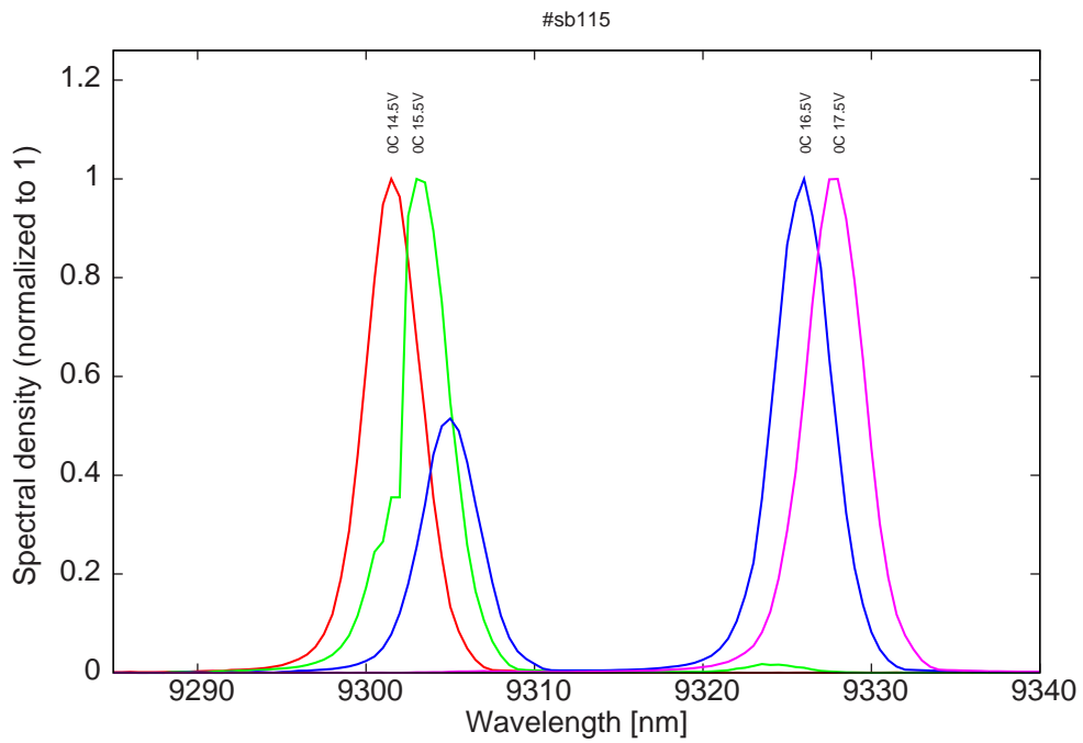
Figure 12: spectra at 0C for various LDD voltages (monomode at threshold and at high LDD voltage)
