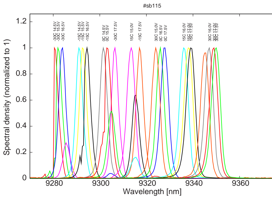
Figure 8: spectra at -30C, -15C, 0C, 15C, and 30C for various LDD voltages
