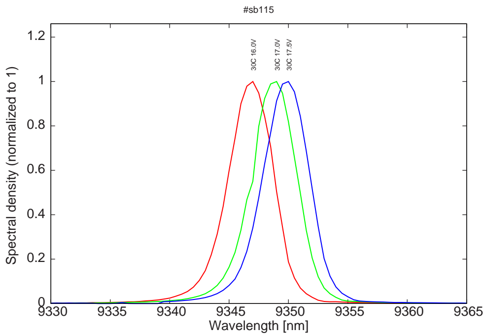
Figure 16: spectra at 30C for various LDD voltages (monomode range at high LDD voltage)
