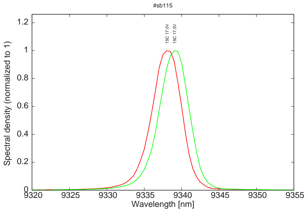
Figure 14: spectra at 15C for various LDD voltages (monomode range at high LDD voltage)
