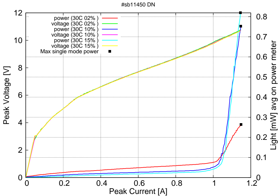
Figure 6: peak voltage and average power vs peak current at 30C for various duty-cycles (200ns pulses on the laser) (the solid squares indicate the maximum singlemode emitted power)
