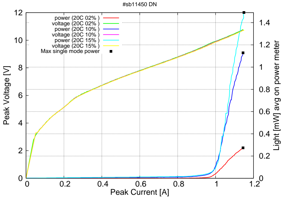
Figure 5: peak voltage and average power vs peak current at 20C for various duty-cycles (200ns pulses on the laser) (the solid squares indicate the maximum singlemode emitted power)
