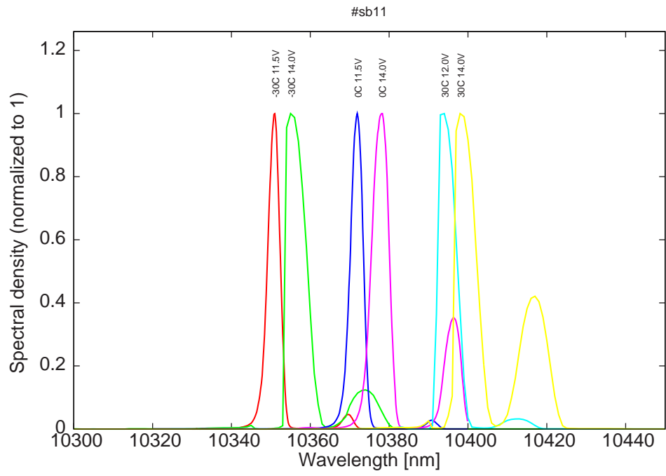
Figure 9: bimode spectra for various temperatures and higher LDD voltages
