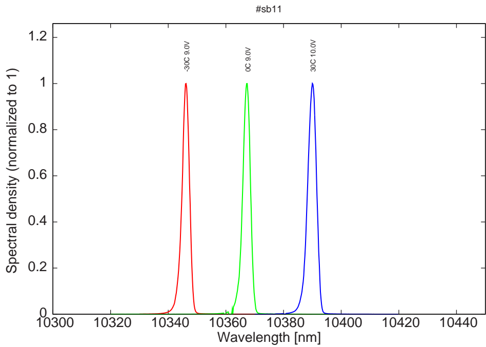
Figure 8: monomode spectra for various temperatures and low LDD voltages
