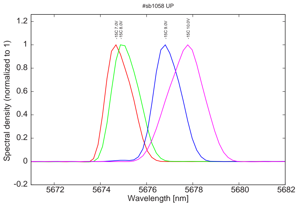
Figure 8: spectra at -15C for various LDD voltages (air absorption around 5676nm)
